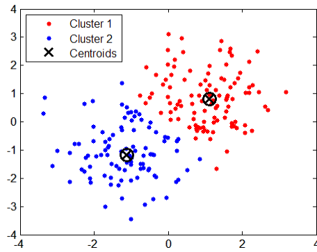
Figure 1: An example of clustering
